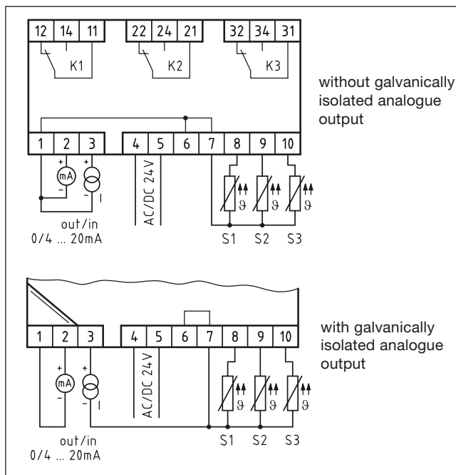
Connection diagram
